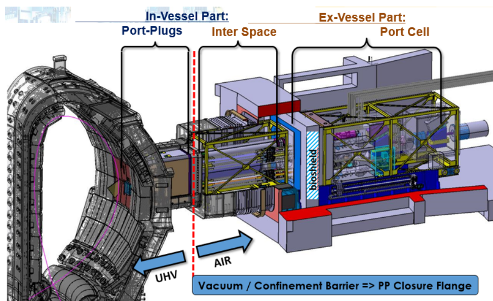
Figure 1. Typical integrated diagnostic port inside ITER infrastructure.
